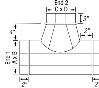
(C) 90° Oval-to-Oval HB Conical
